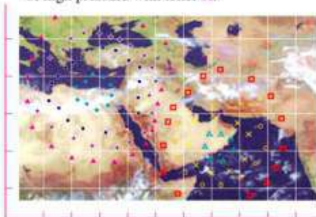
Atmospheric pressure map Figure (4)
